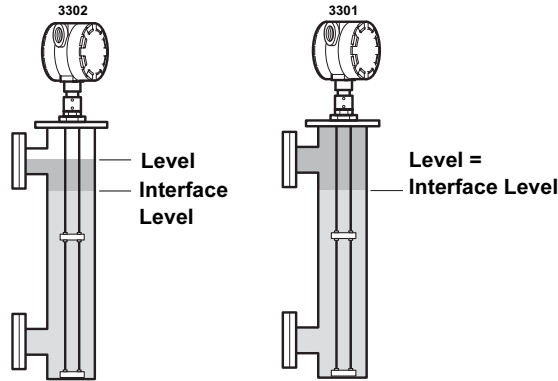
Interface Measurement with Model 3302 and 3301 (fully immersed probe).
